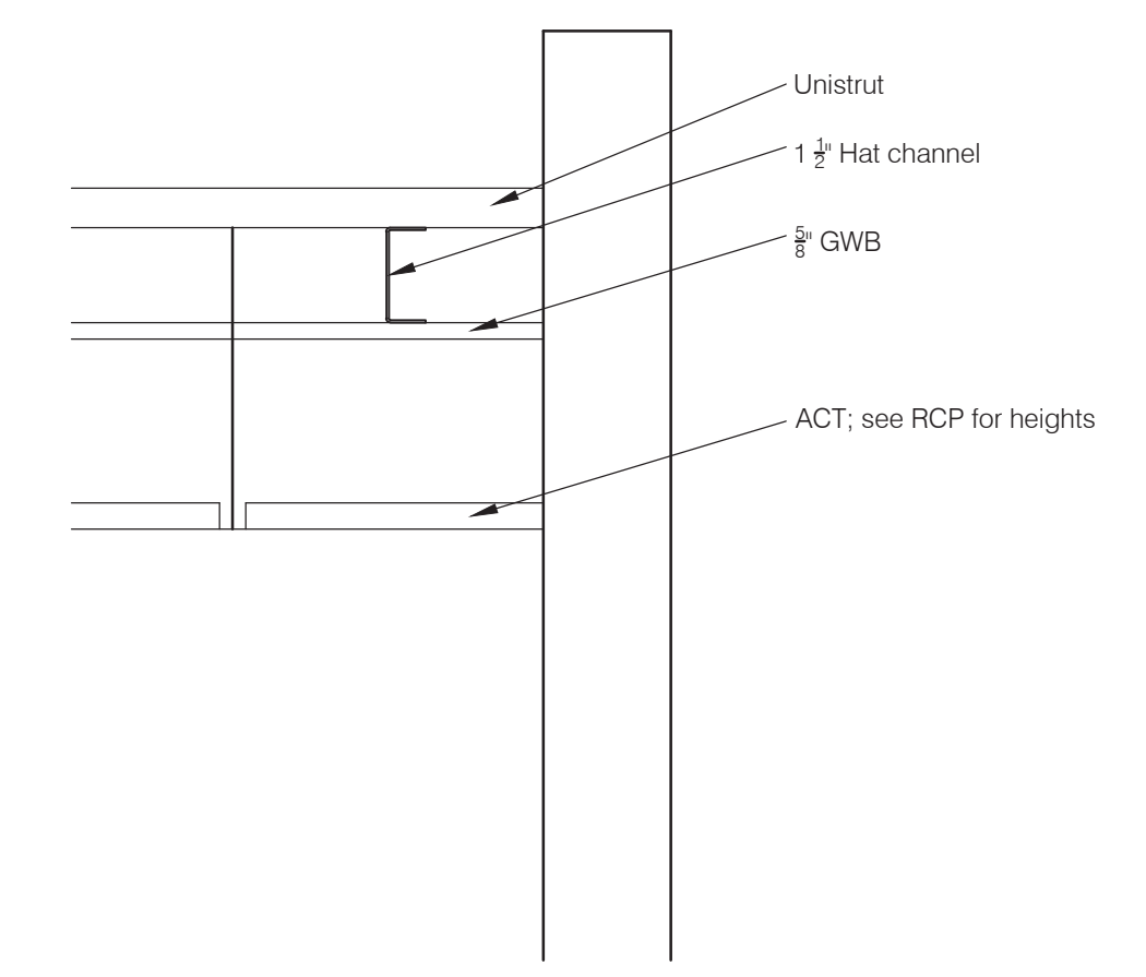
2 Ceiling Detail 1 1/2" = 1'-0"
